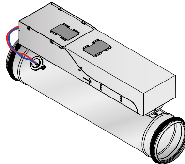
Figur 1. WISE Cover Circular Damper.
