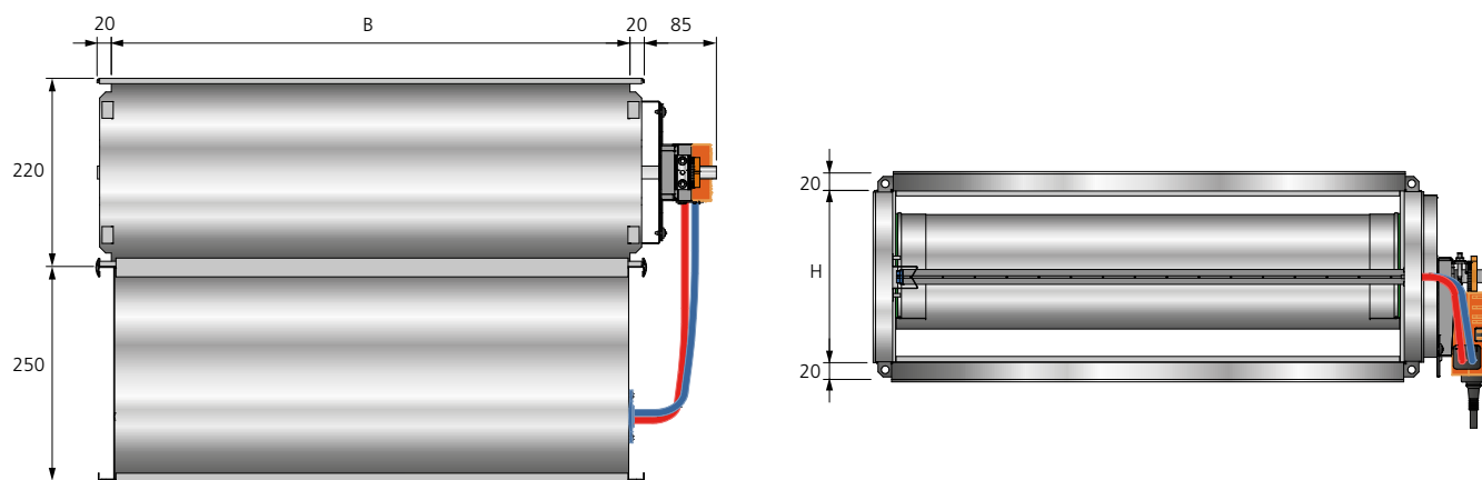
Figure 5. Dimensions (mm), REACT V BBAC rectangular.
