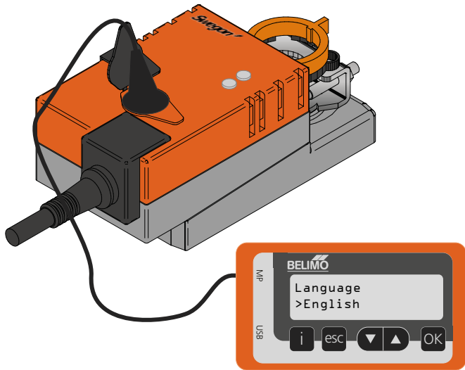
Figure 10. ZTH EU – Hand-held terminal for setting and reading the actuator's parameters.
